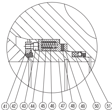
BI - DIRECTIONAL SEAT DOUBLE - PISTON
