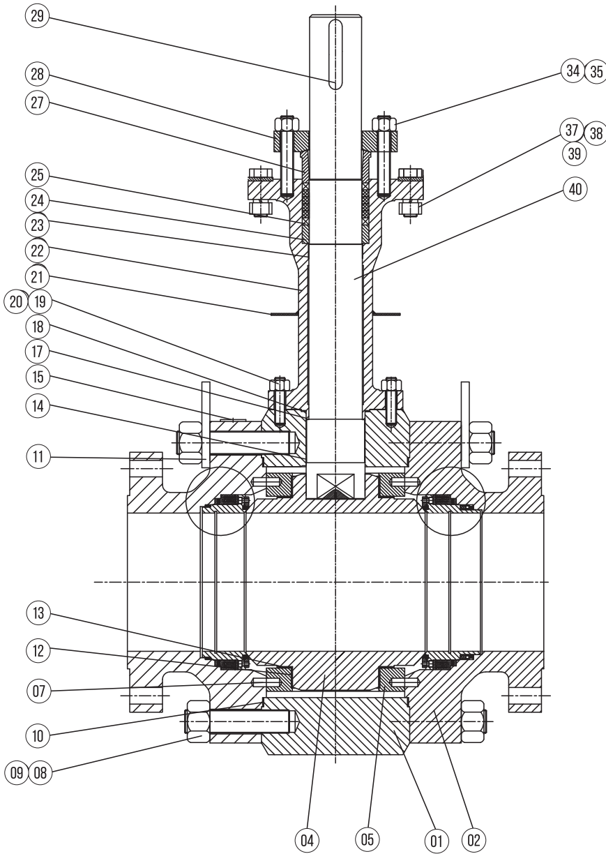
BI - DIRECTIONAL SEAT DOUBLE - PISTON
