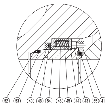
UNI - DIRECTIONAL SEAT SINGLE - PISTON
